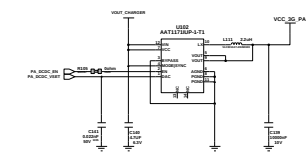
<DC DC CONVERTER FOR 3G PAD >
