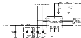
<3G PAM Band1 2100>
